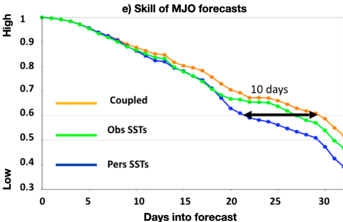
Fig. 4. Atmospheric convection perturbation (outgoing longwave radiation, contours every 10 \text{ W m}^{-2} ) and sea surface temperature (SST; colors) composites of two successive phases of (a),(b) the Madden–Julian oscillation (MJO) during December–March and (c),(d) the monsoon intraseasonal oscillation (MISO) during June–September. (e) MJO forecast skill as a function of lead time (days) for forecasts with fixed SST, observed SST, and active ocean–atmosphere coupling. The MJO and MISO modulate tropical rainfall during boreal winter and summer, respectively. They are associated with SST and oceanic mixed layer processes, which need to be better observed to improve their forecasts.
